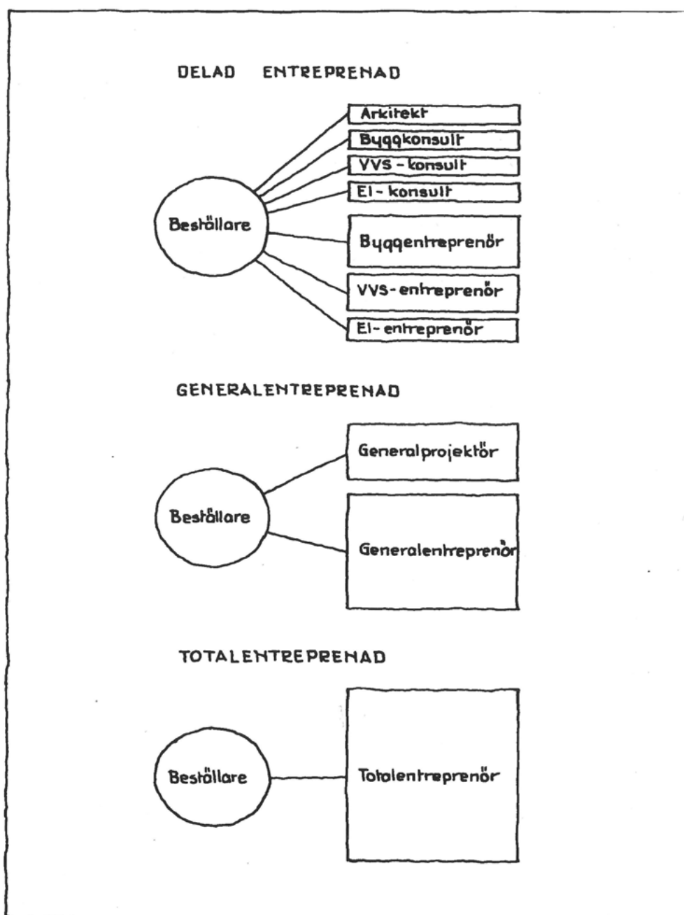
Fig. 1:6 Entreprenadformer, principalschema.
